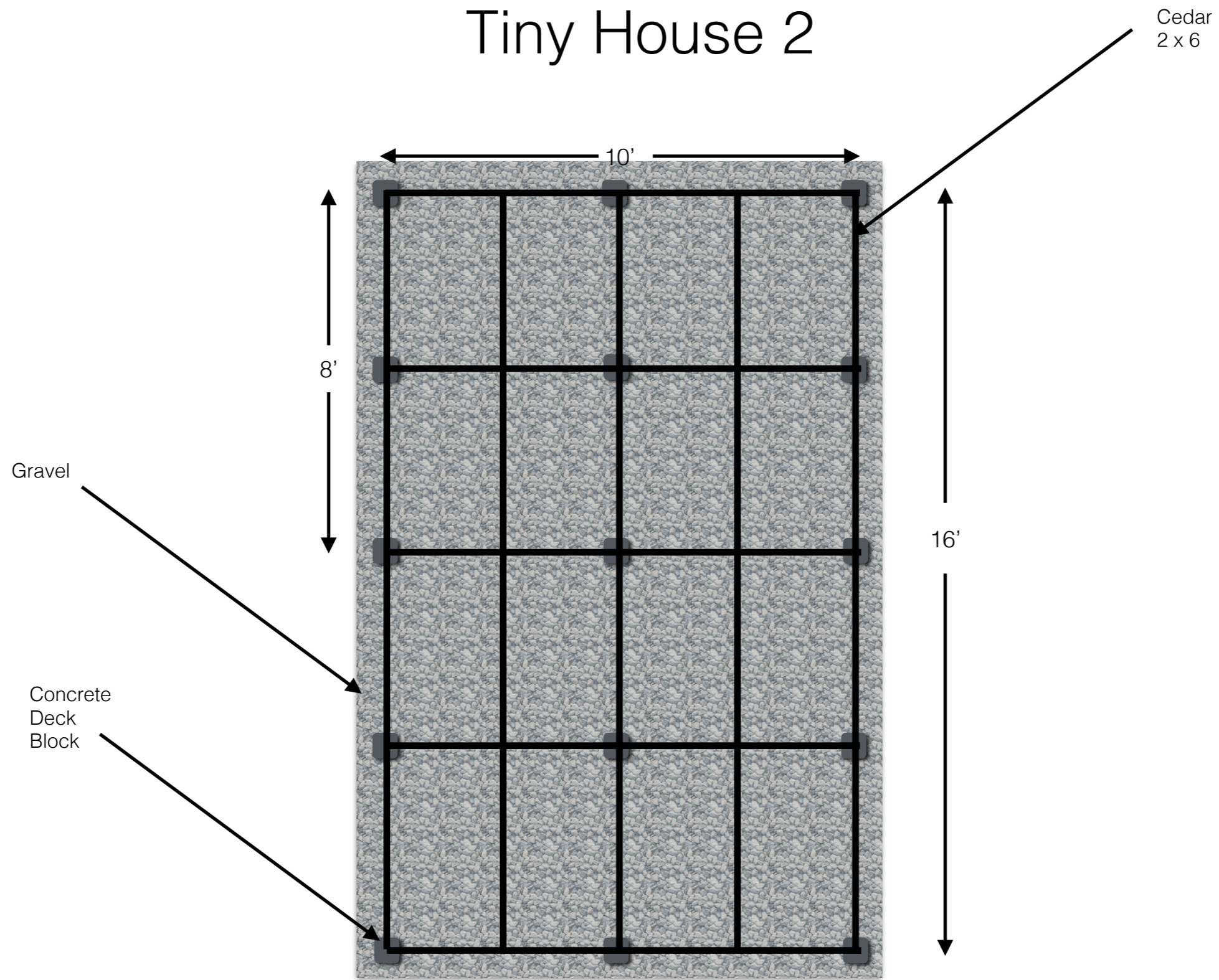
Deck Base Plan View
